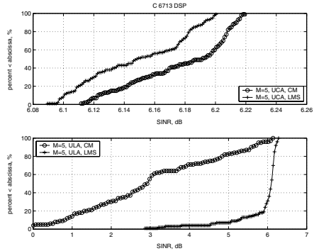
Fig. 9. Cumulative distribution of received SINR for the beamformer implementation on C6713 DSP
