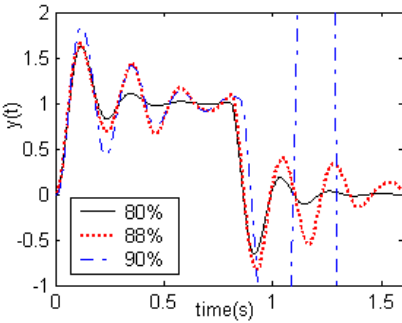
Fig. 4. System responses over CAN, with different r_o values
