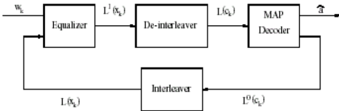
Fig. 4. Receiver model for Turbo equalizer
