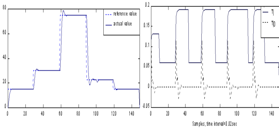
Fig. 7. The response to different values (25, 50, 75 rad/sec) of the reference signal, and the matched learning rate
