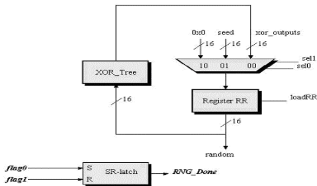
Fig. 2. A 16-bit random generator architecture
