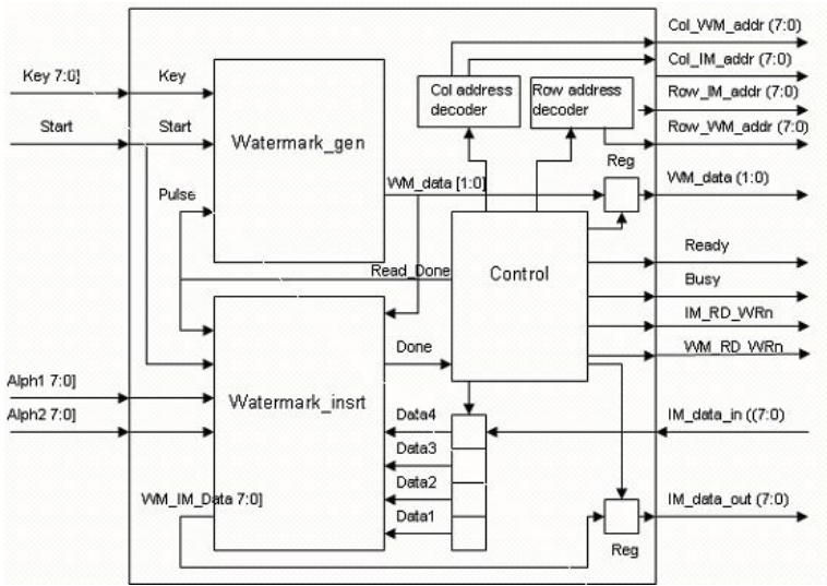
Fig. 1. Datapath and Controller for the Proposed Chip.
