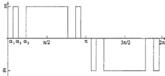
Fig. 1. A symmetric three-level PWM waveform.
