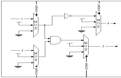
Fig. 7. The fault injection scheme in hardware
