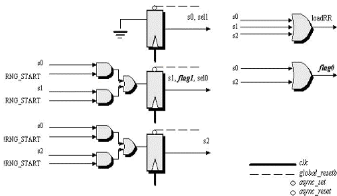
Fig. 3. Internal structure of the random generator
