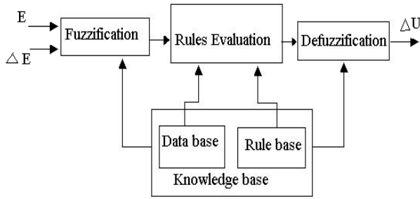
Fig. 2. Block diagram of the fuzzy inference system
