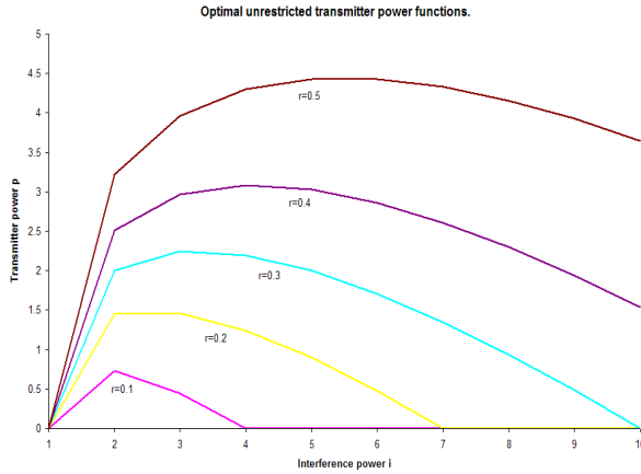
Fig. 4. The Power at various interference ratios [9], [12], [20]
